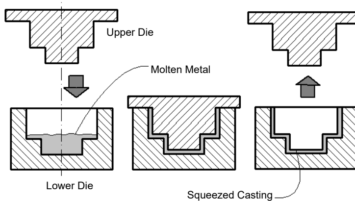
Fig. 5.8: Squeeze Casting
