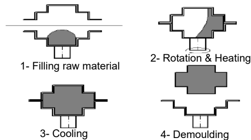
Fig 4.36: Rotational Moulding
