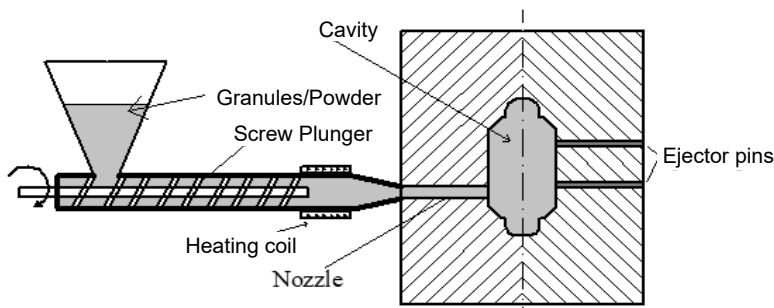
Fig. 4.35: Injection Moulding
