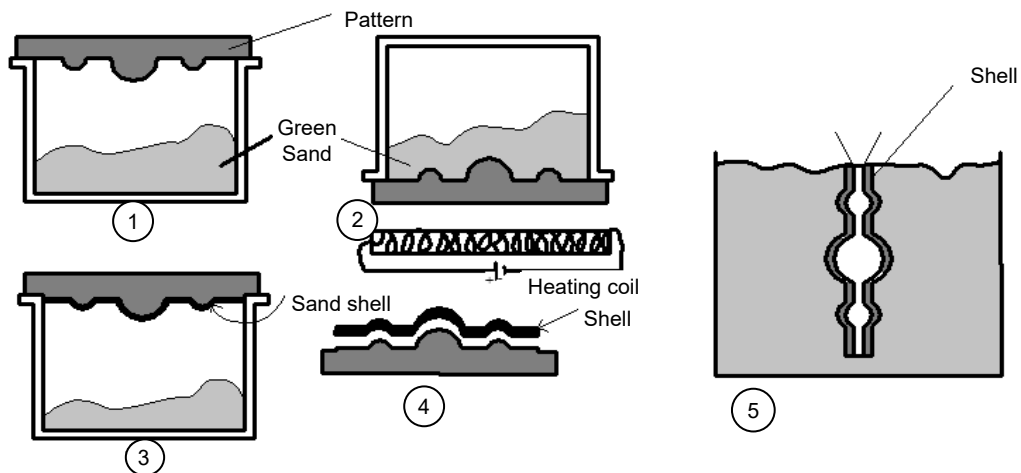
Fig. 5.3: Shell Casting
