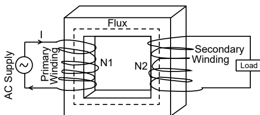
Fig. 3.6: Transformer
